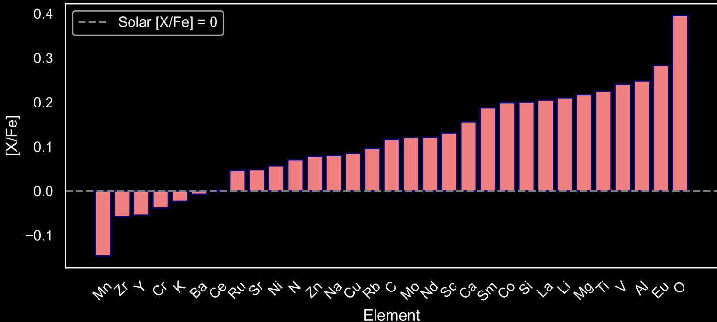
Abundance Pattern for GALAH Red Giants: Star Field [23] (N=61)
