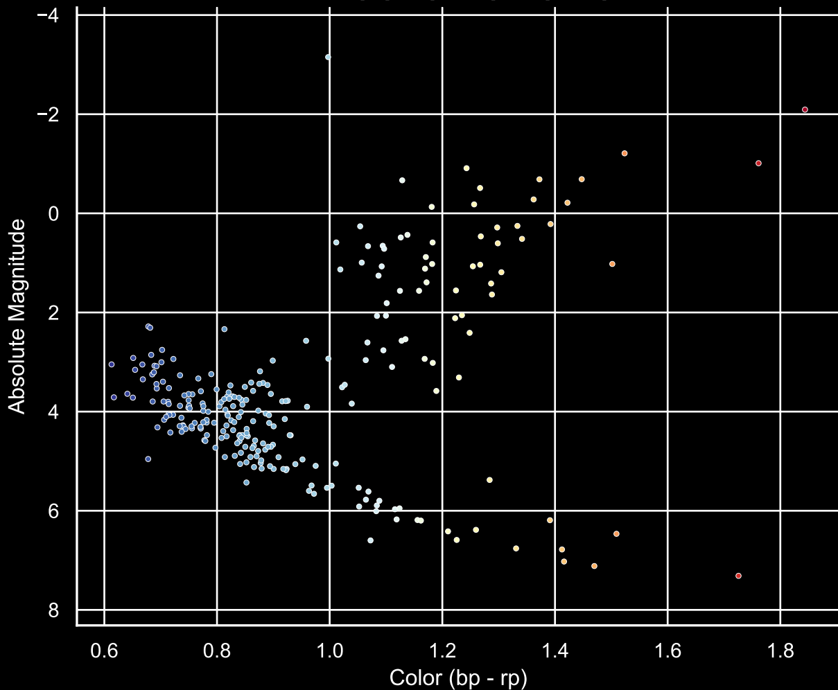
GALAH Hertzprung-Russel Diagram Field [23] Ra [329.36] Dec [-58.37]
