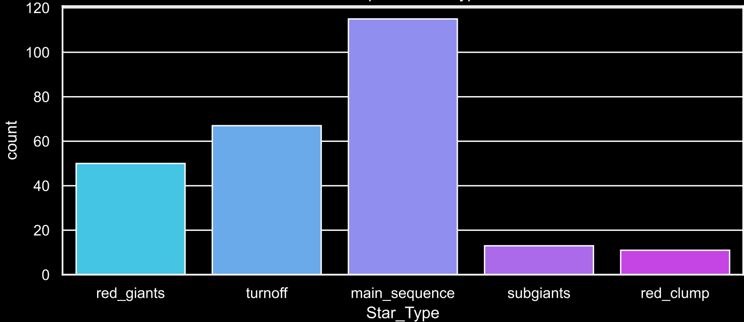
Field [23] Count plot of Star Type
