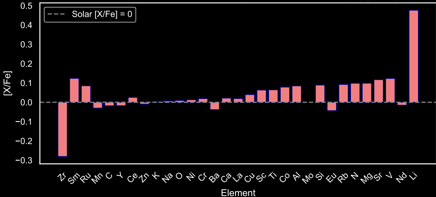
Abundance Pattern for GALAH Main Sequence Stars: Star Field [23] (N=115)
