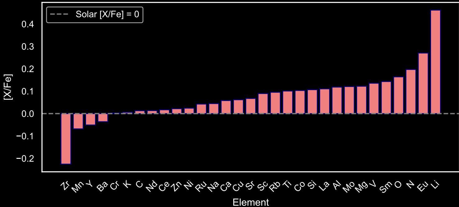
Abundance Pattern for GALAH Star Field [23] (N=256)
